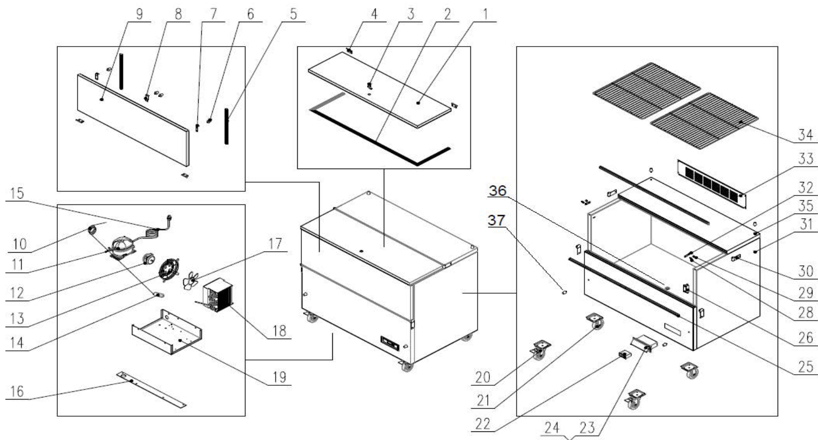
EXPLODE OF KCHMC49
